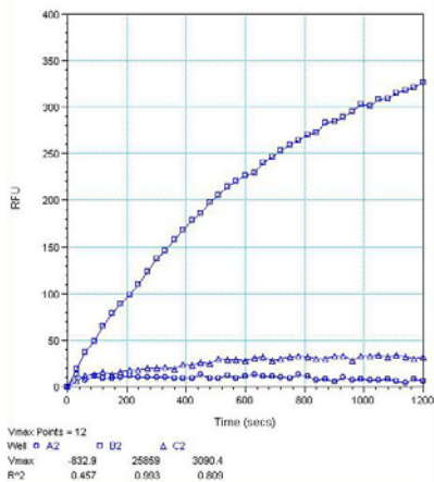
Figure 2. GTP-exchange assay with KRas4B G13D and SOS1.
