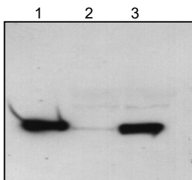
Figure 3: Control Assay Results for Rac1 Activation Assay
