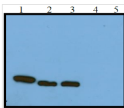
Figure 3: Control Assay Results for Cdc42 Activation Assay
