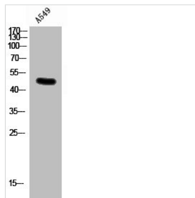
Western Blot analysis of A549 cells using Connexin 47 Polyclonal Antibody
