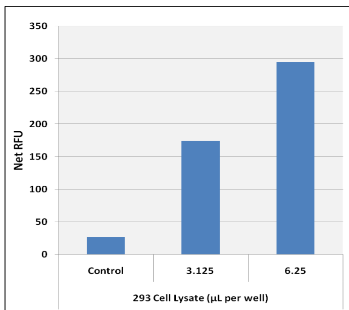
Figure 3: 2-PG detection in 293 Cells using the 2-Phosphoclygerate Assay Kit (Fluorometric). Cells were homogenized and deproteinated according to the preparation of samples section above.
