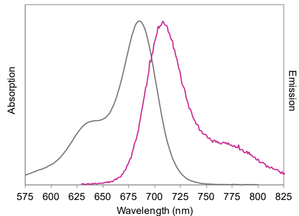
Absorption and emission spectra of NucSpot® 680 with DNA.
