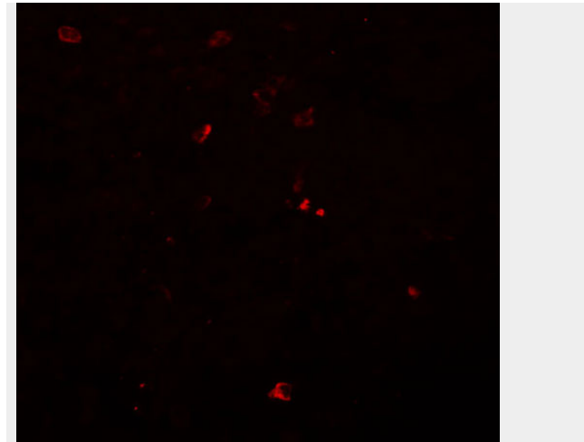
Immunofluorescence of BCAS3 in human breast carcinoma tissue with BCAS3 antibody at 20 µg/mL.
