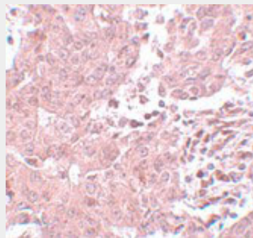
Immunohistochemistry of BCAS3 in human breast carcinoma with BCAS3 antibody at 5 µg/mL.
