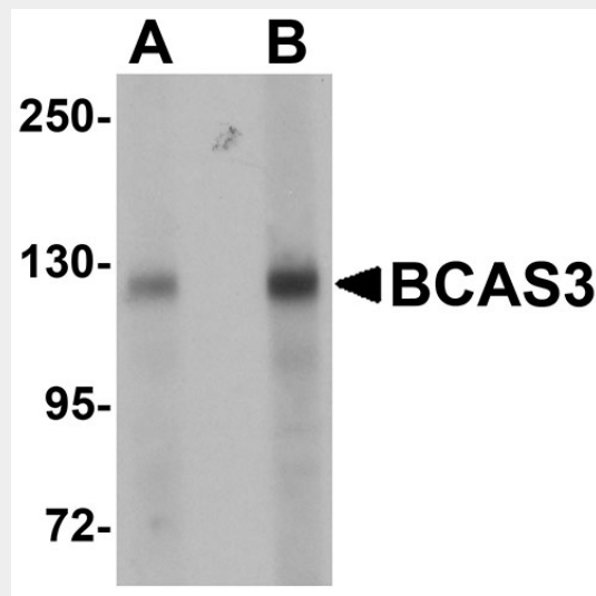
Western blot analysis of BCAS3 in rat brain tissue lysate with BCAS3 antibody at (A) 0.5 and (B) 1 µg/mL.
