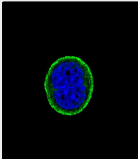
Confocal immunofluorescent analysis of IL10RA Antibody (Center)(Cat#AP8768c) with MCF-7 cell followed by Alexa Fluor® 488-conjugated goat anti-rabbit IgG (green). DAPI was used to stain the cell nuclear (blue).
