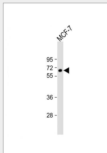
Anti-IL10RA Antibody (Center) at 1:1000 dilution + MCF-7 whole cell lysate Lysates/proteins at 20 µg per lane. Secondary Goat Anti-Rabbit IgG, (H+L), Peroxidase conjugated at 1/10000 dilution. Predicted band size : 63 kDa
