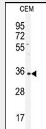
Western blot analysis of IGHAI antibody (C-term) (Cat.#AP7456b) in CEM cell line lysates (35ug/lane). IGHAI (arrow) was detected using the purified Pab .
