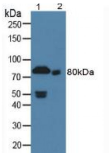
Western blot analysis of (1) Rat Serum and (2) Rat Liver Tissue.
