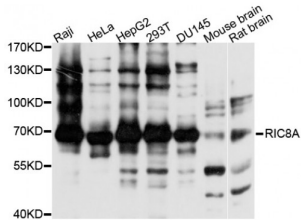
Western blot analysis of extracts of various cell lines, using RIC8A antibody (abx126481) at 1/1000 dilution.
