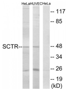
Western blot analysis of extracts from HeLa cells and HUVEC cells, using SCTR antibody.
