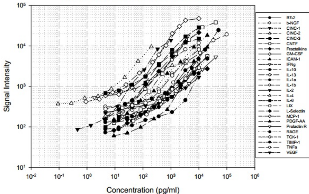
QAR-CYT-3 Standard Curves
