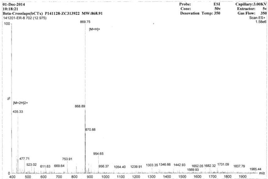
Figure 2. MASS Spectrometry
