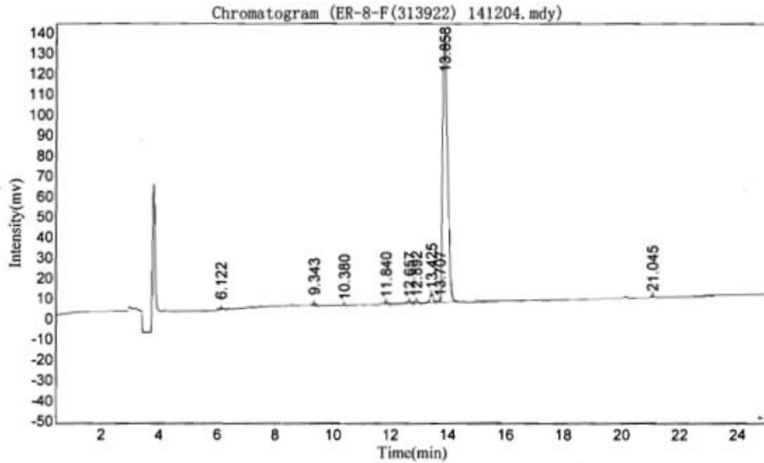
Figure 1. HPLC
