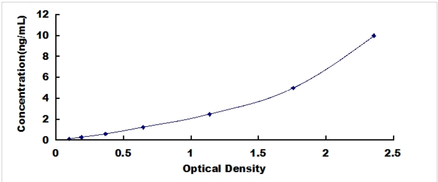
Typical Standard Curve for PRKG1, Mouse ELISA.
