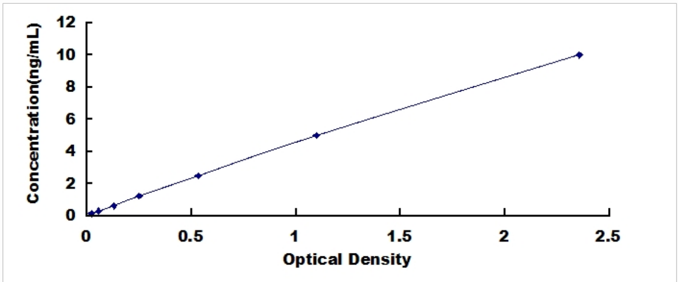
Typical Standard Curve for PPOX, Human ELISA.
