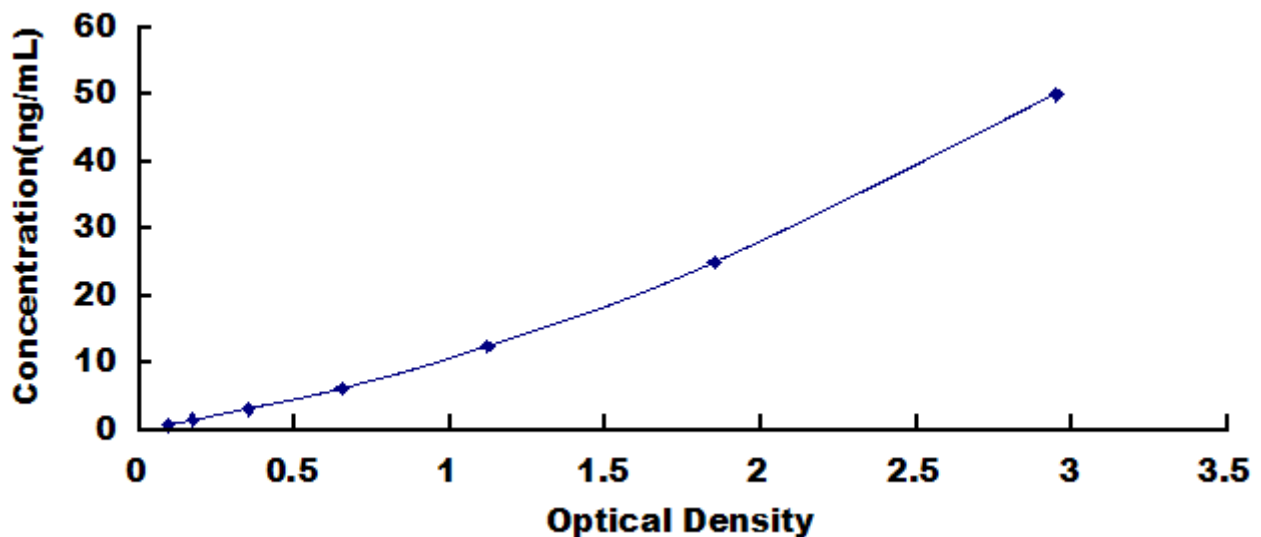
Typical Standard Curve for ALDH3A1, Human ELISA.
