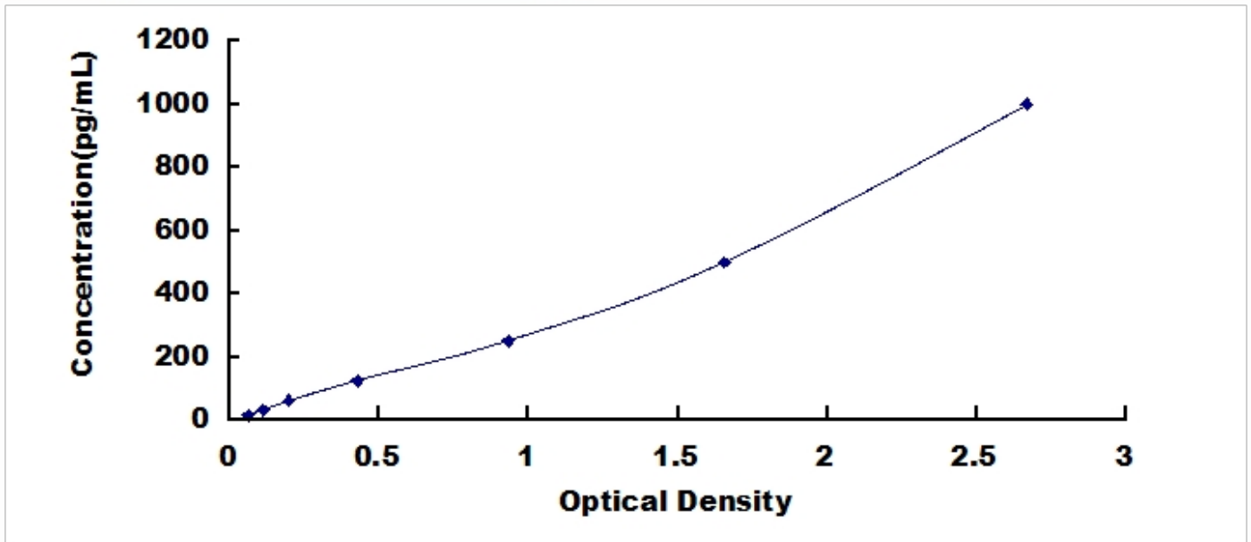
Typical Standard Curve for PGLYRP2, Human ELISA.
