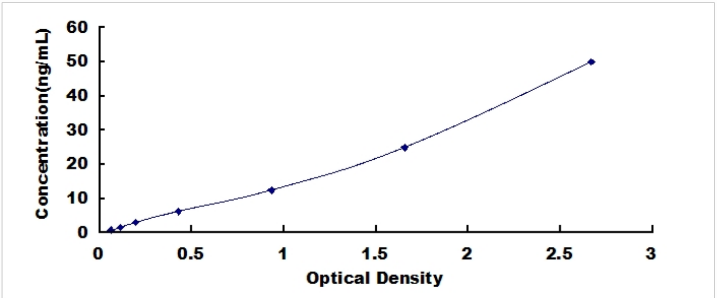
Typical Standard Curve for ASNS, Human ELISA.
