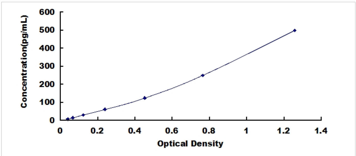
Typical Standard Curve for FGF21, Human ELISA.
