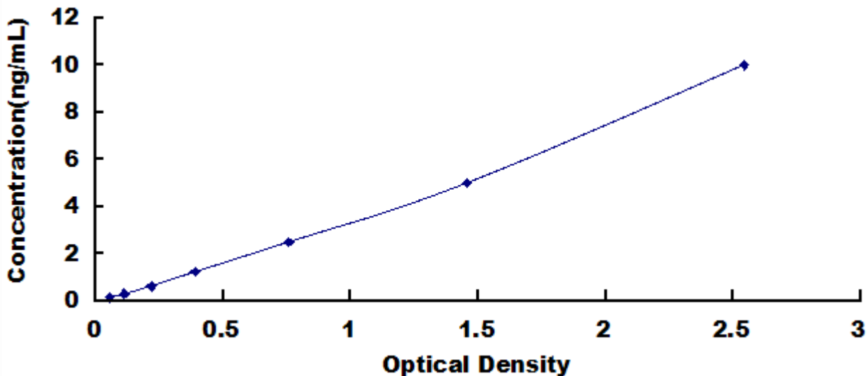
Typical Standard Curve for TST, Mouse ELISA.
