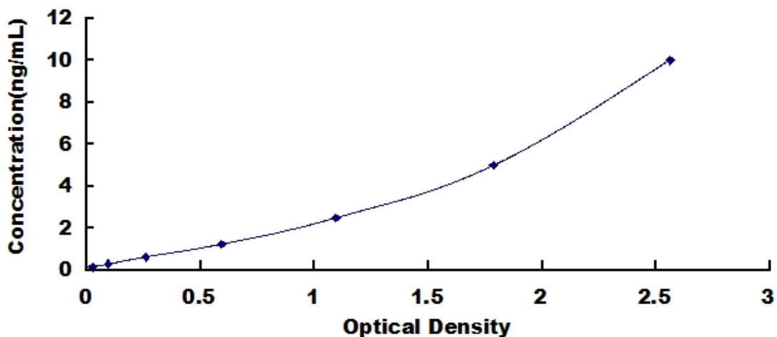
Typical Standard Curve for C5b-9, Rat ELISA.
