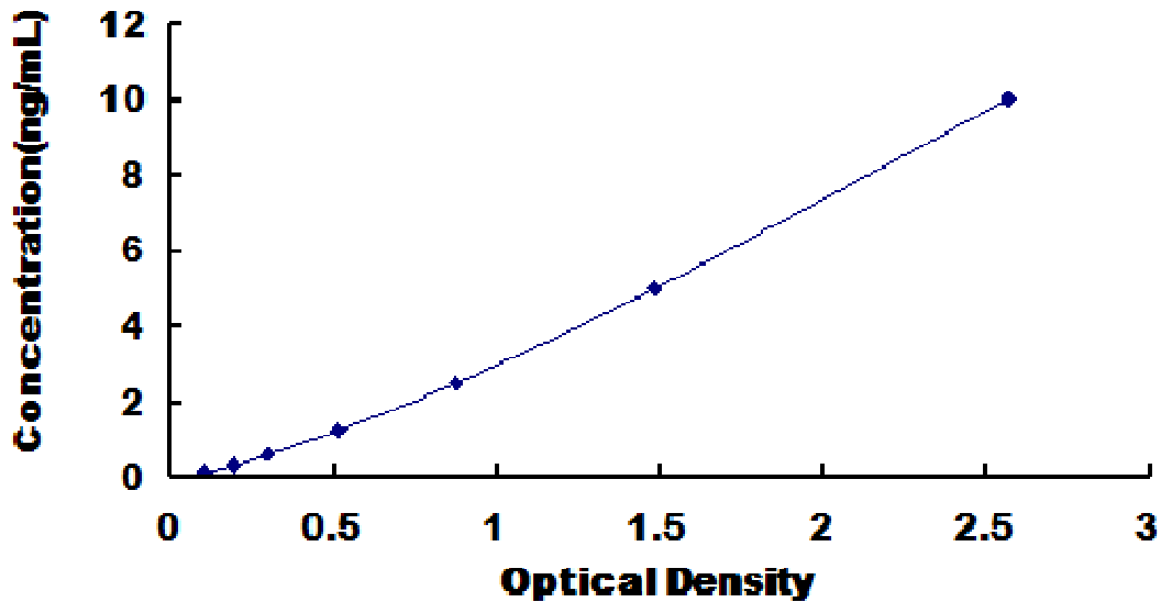
Typical Standard Curve for ASPN, Mouse ELISA.
