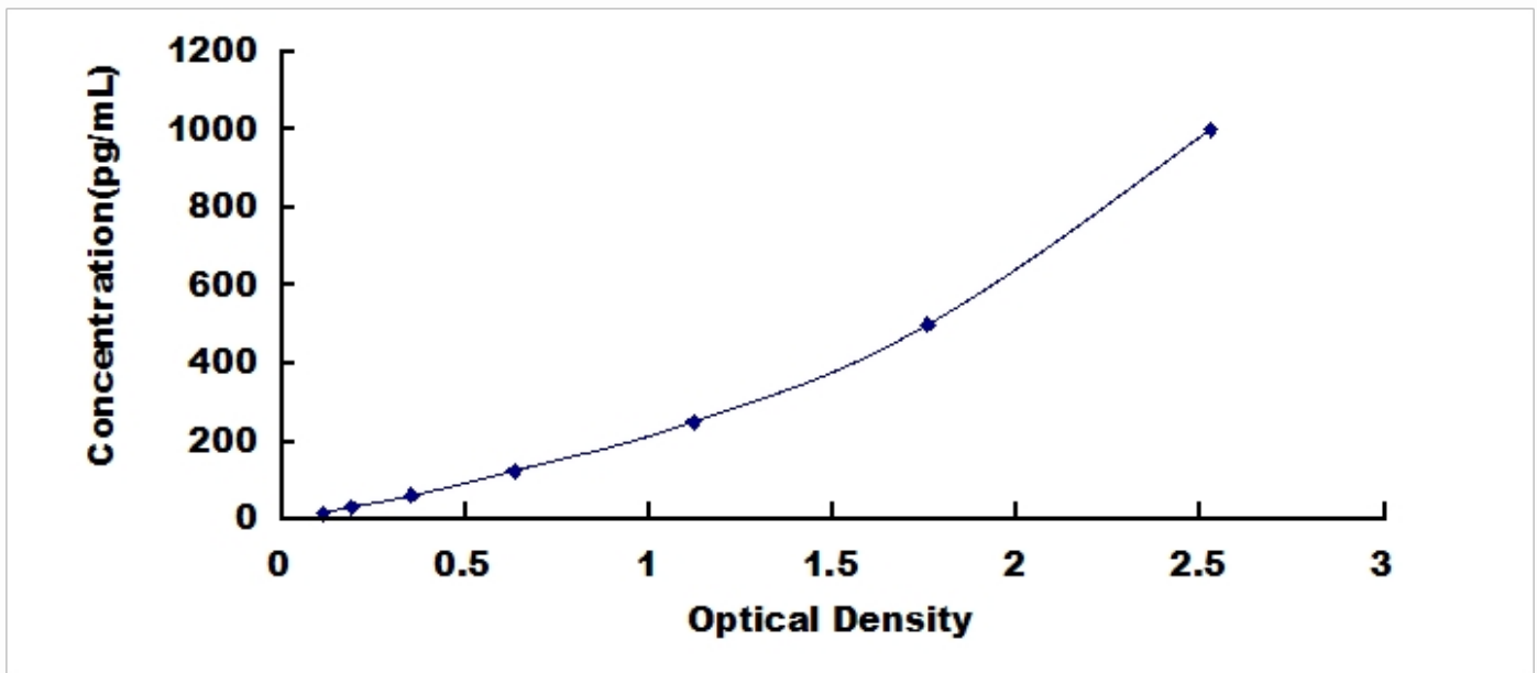
Typical Standard Curve for TARC, Rat ELISA.
