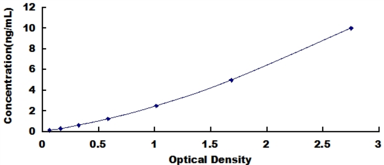
Typical Standard Curve for TNFRSF4, Human ELISA.
