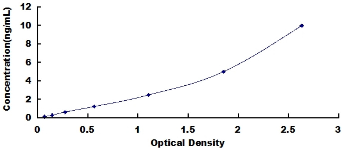
Typical Standard Curve for TSPAN30, Human ELISA.
