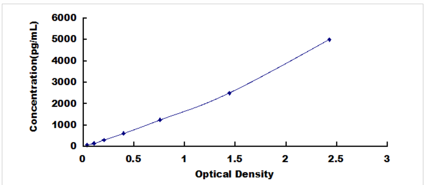
Typical Standard Curve for APP, Human ELISA.
