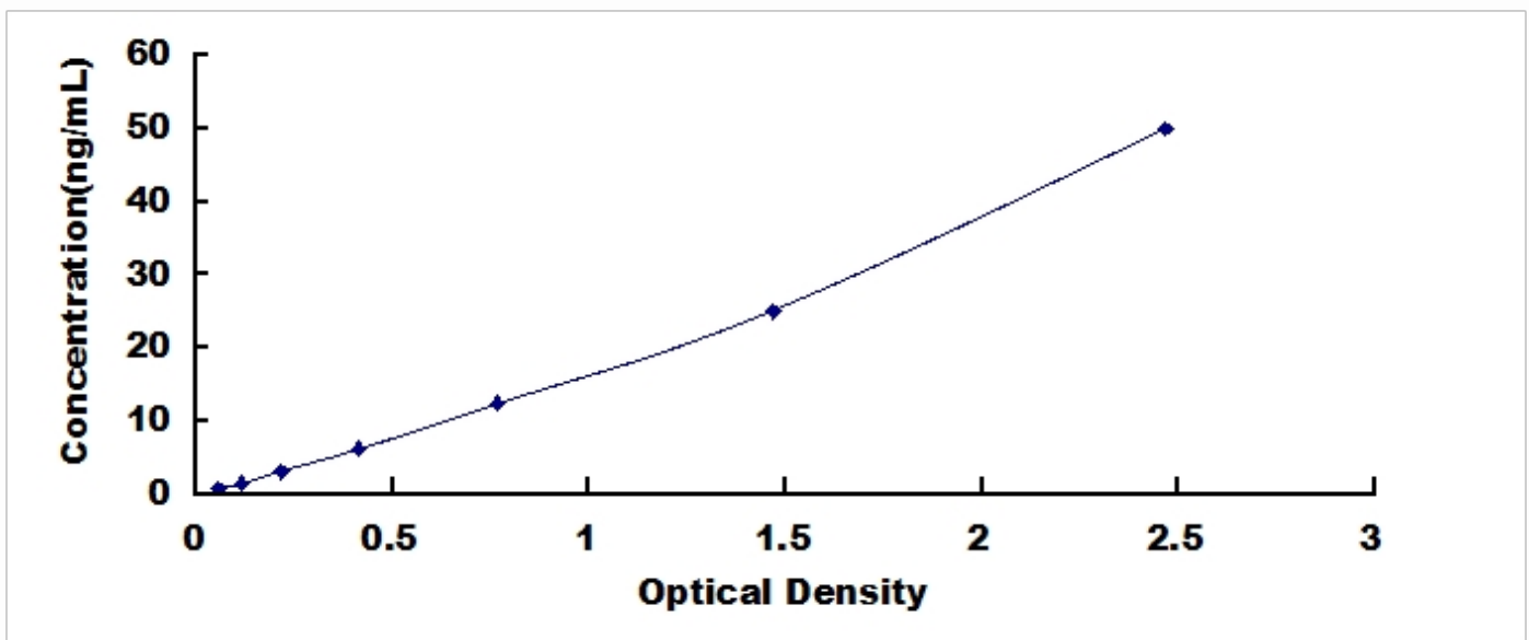
Typical Standard Curve for Ceruloplasmin, Mouse ELISA.
