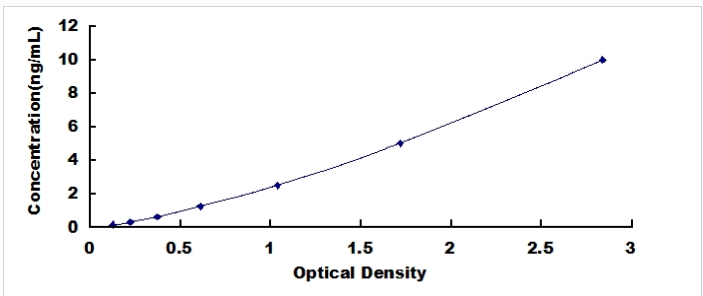
Typical Standard Curve for CA2, Human ELISA.
