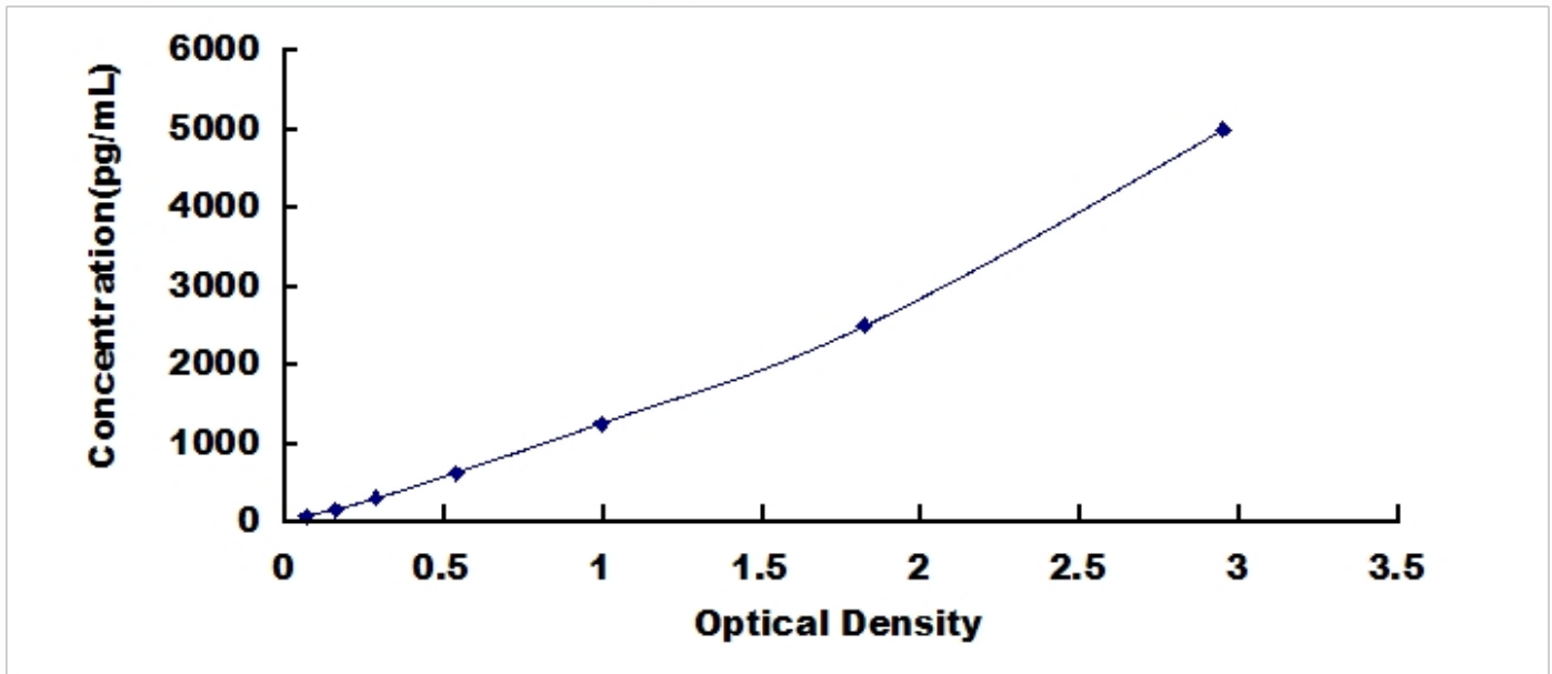
Typical Standard Curve for MUC5AC, Human ELISA.
