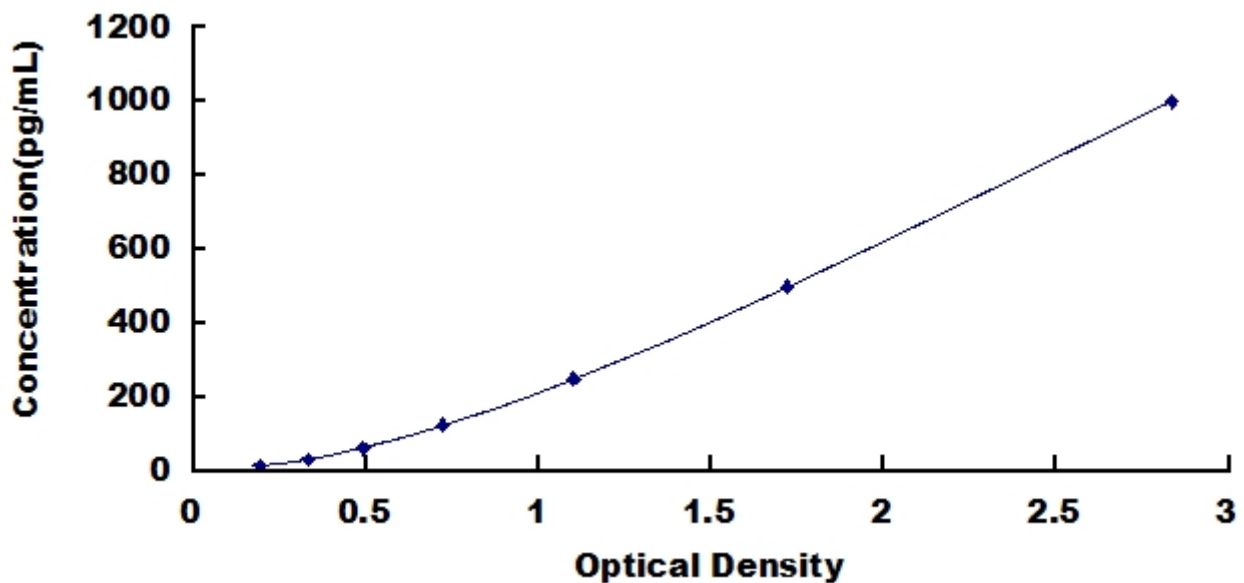
Typical Standard Curve for GDF9, Human ELISA.
