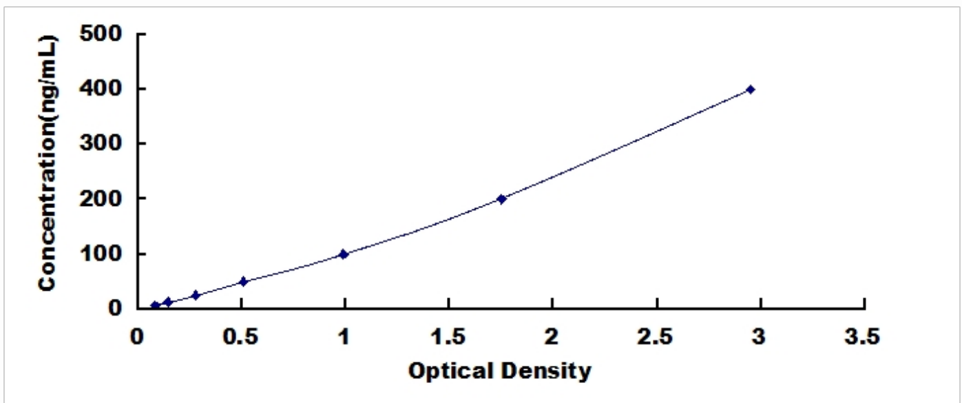
Typical Standard Curve for Gelsolin, Human ELISA.
