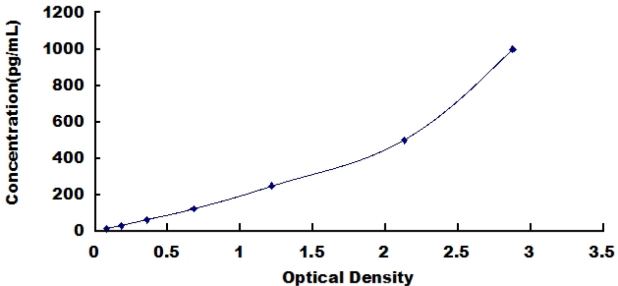
Typical Standard Curve for IL17, Rat ELISA.
