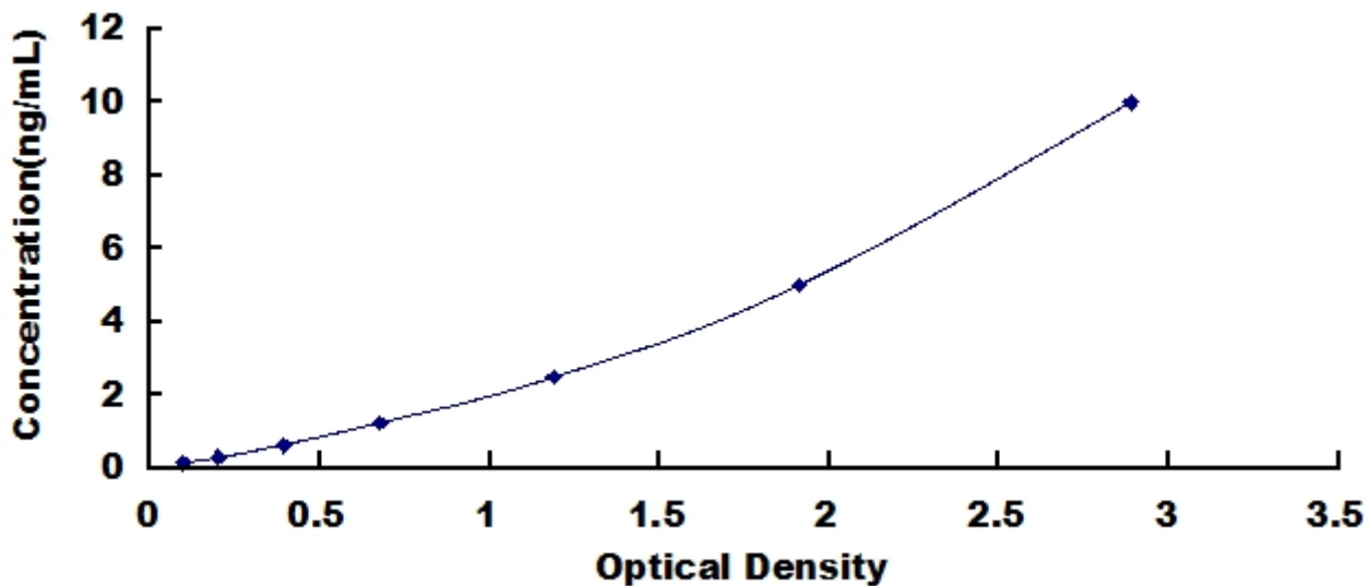
Typical Standard Curve for GH, Human ELISA.
