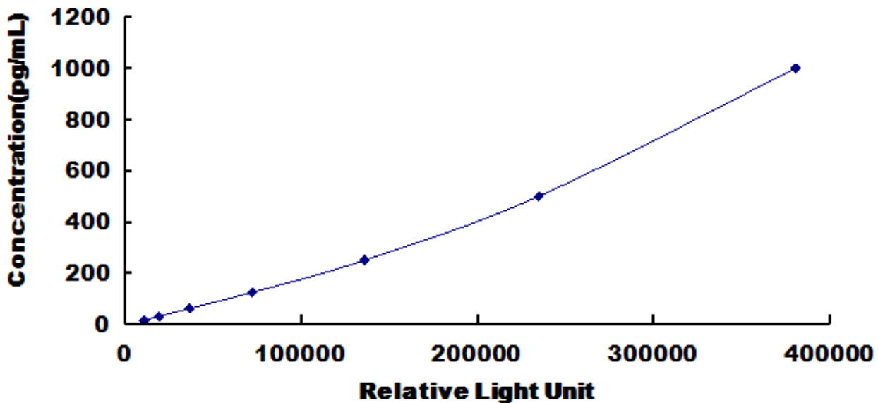
Typical Standard Curve for Human GKN2 CLIA.
