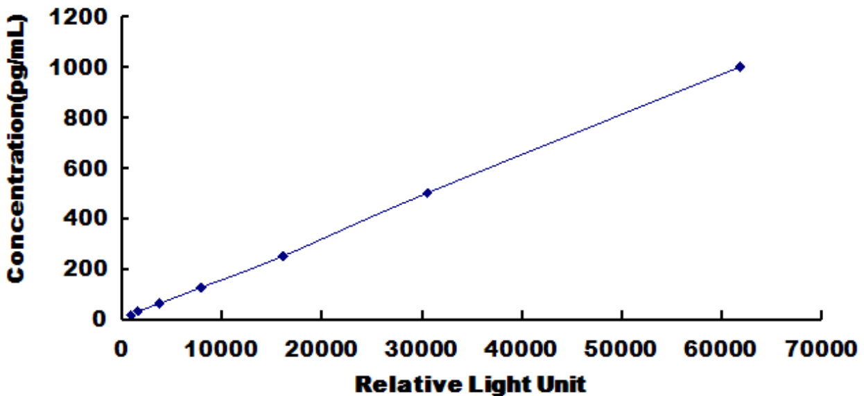
Typical Standard Curve for Human IFNa21 CLIA.
