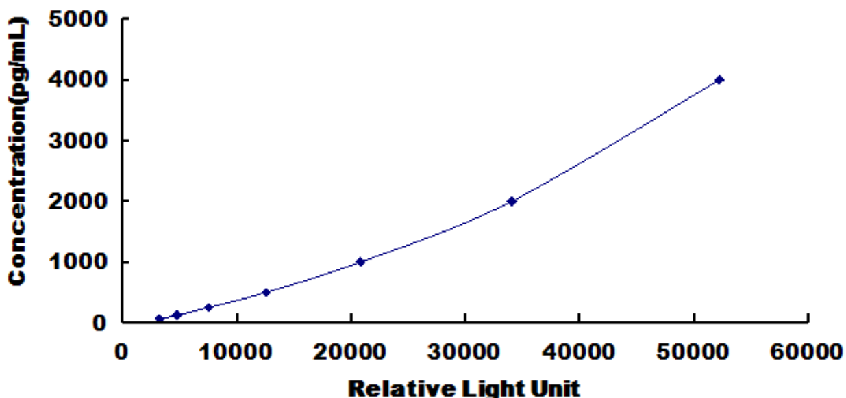
Typical Standard Curve for Rat GDF3 CLIA.
