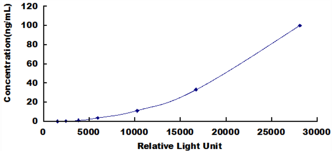
Typical Standard Curve for Osteopontin, Human CLIA.
