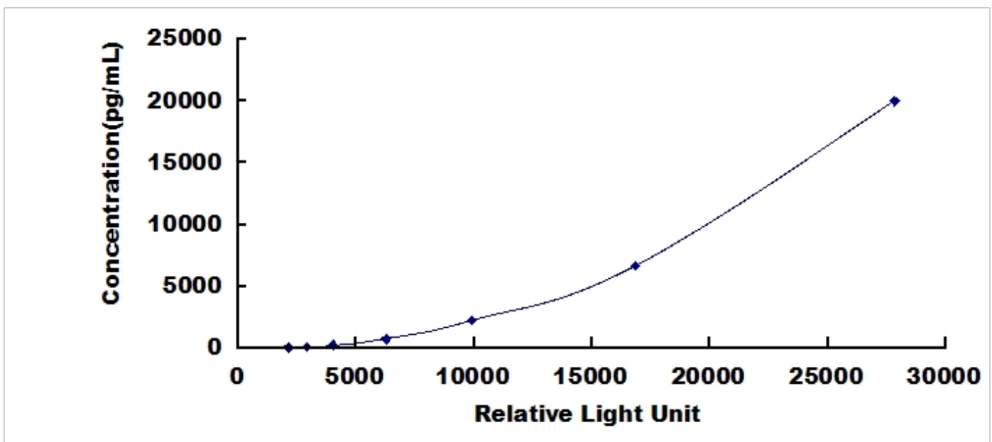
Typical Standard Curve for C3a, Human CLIA.
