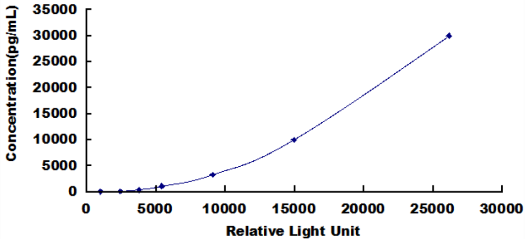
Typical Standard Curve for Leptin, Mouse CLIA.
