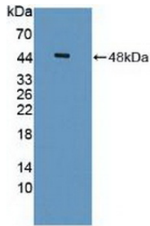
Figure. Western Blot; Sample: Recombinant ISLR, Human.
