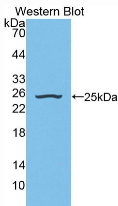
Used in Western Blot, Sample: Recombinant SIAL2, Rat
