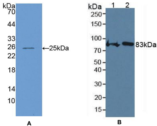
Figure 1. Western Blot
