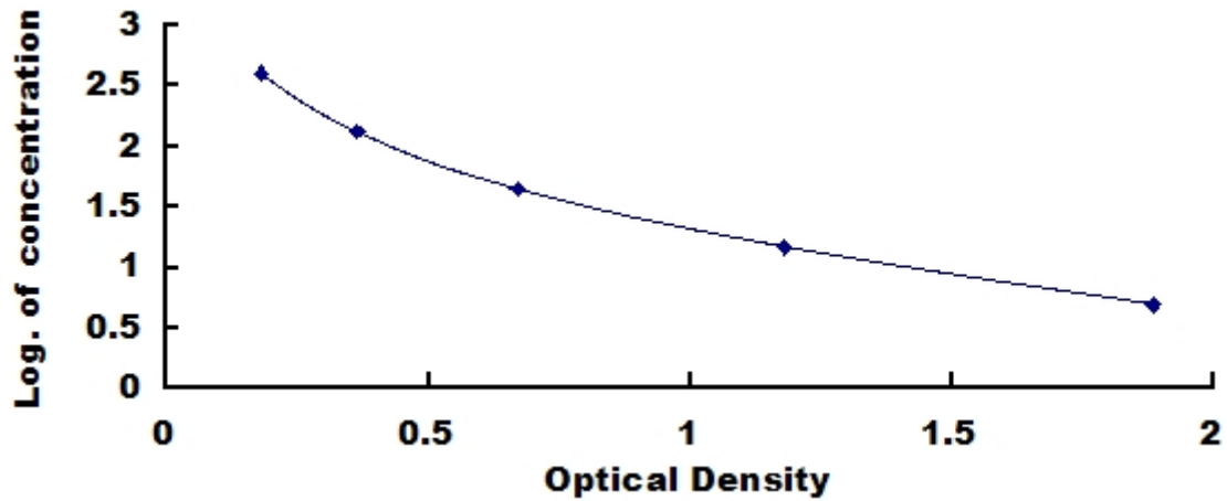
Typical Standard Curve for NEFL, Mouse ELISA.
