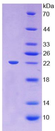
Figure 2. SDS-PAGE
