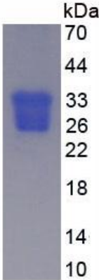
Figure 2. SDS-PAGE
