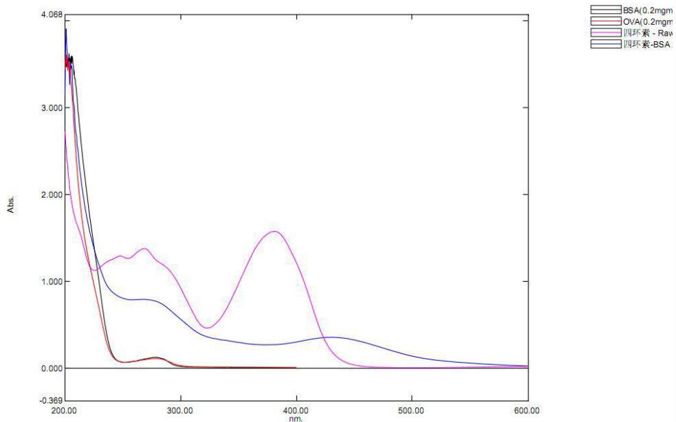
Figure 2. UV-spectrum
