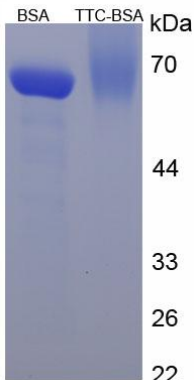
Figure 1. SDS-PAGE
