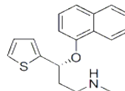
Chemical Structure
