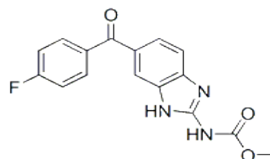
Chemical Structure
