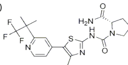
Chemical Structure
